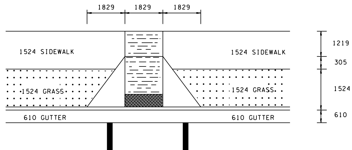
TANGENT SECTION WITH 1524 mm GRASS STRIP
