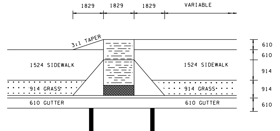
TANGENT SECTION WITH 914 mm GRASS STRIP
